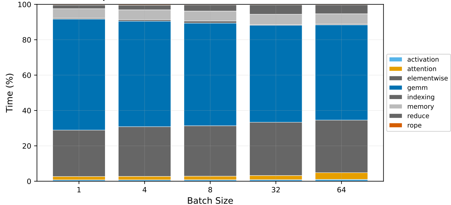
Qwen3-32B — decode Kernel Time Breakdown
