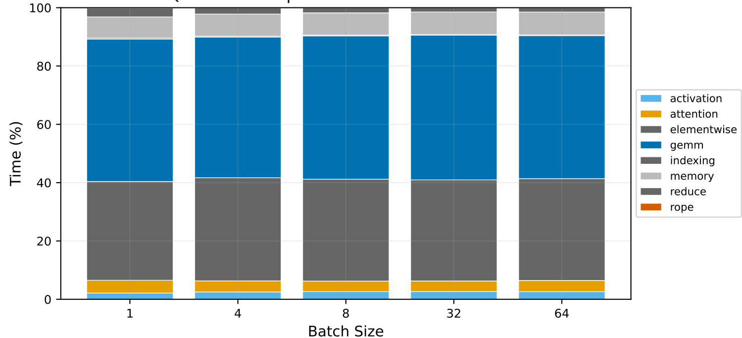
Qwen3-32B — prefill Kernel Time Breakdown
