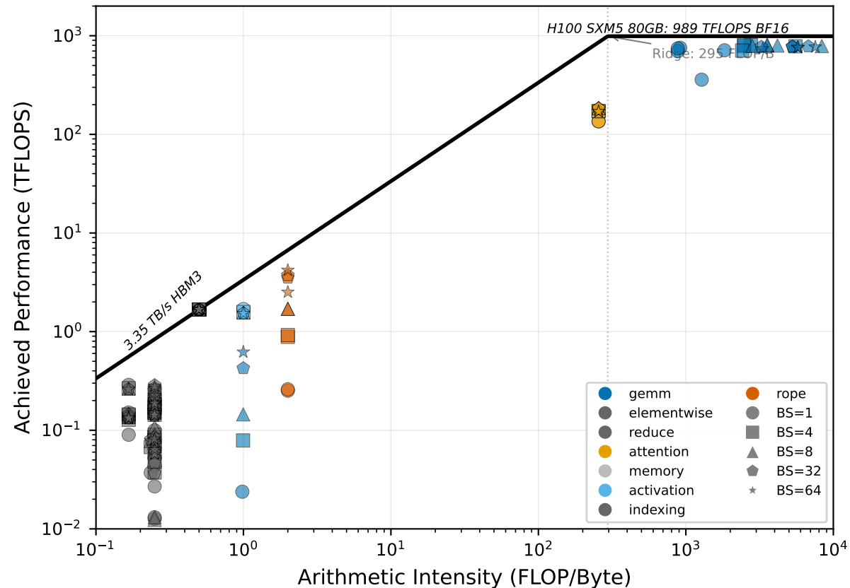
Qwen3-32B — prefill (batch size sweep)
