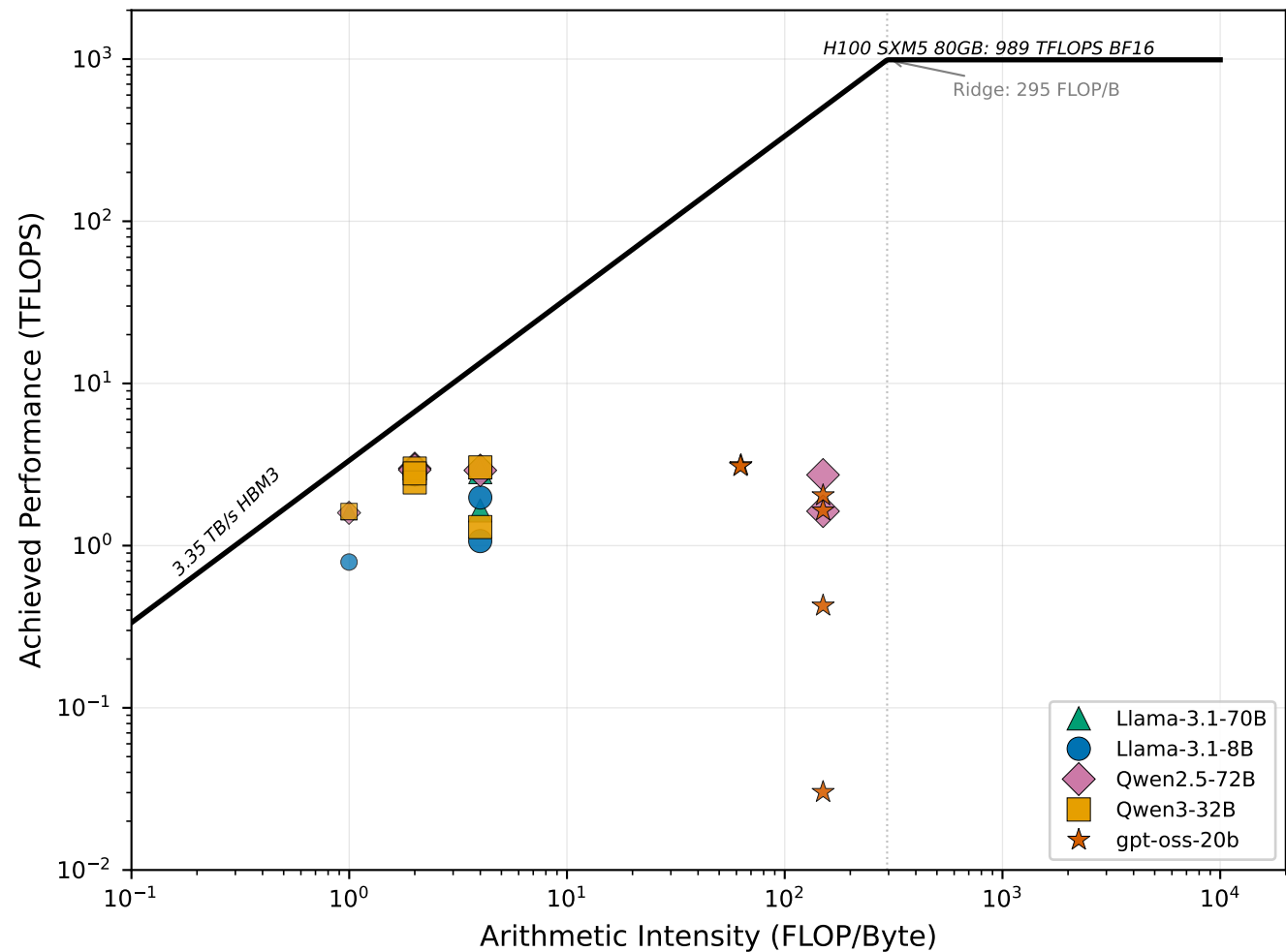
Cross-Model Roofline — decode (BS=1)
