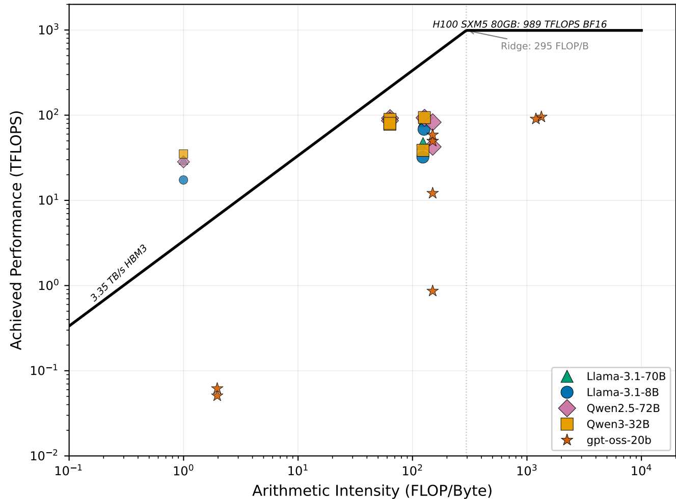
Cross-Model Roofline — decode (BS=32)
