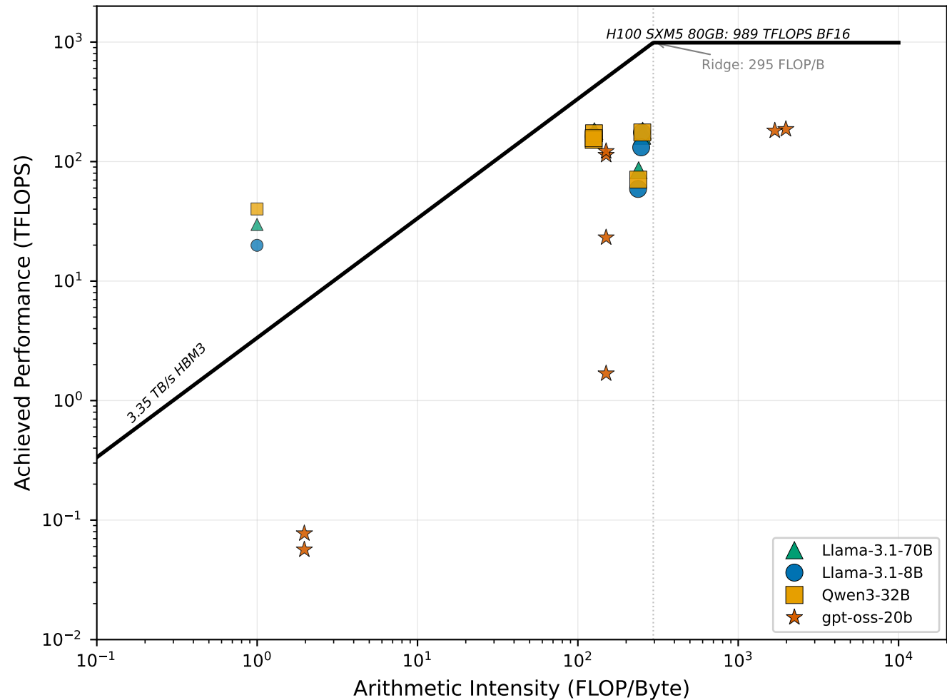
Cross-Model Roofline — decode (BS=64)
