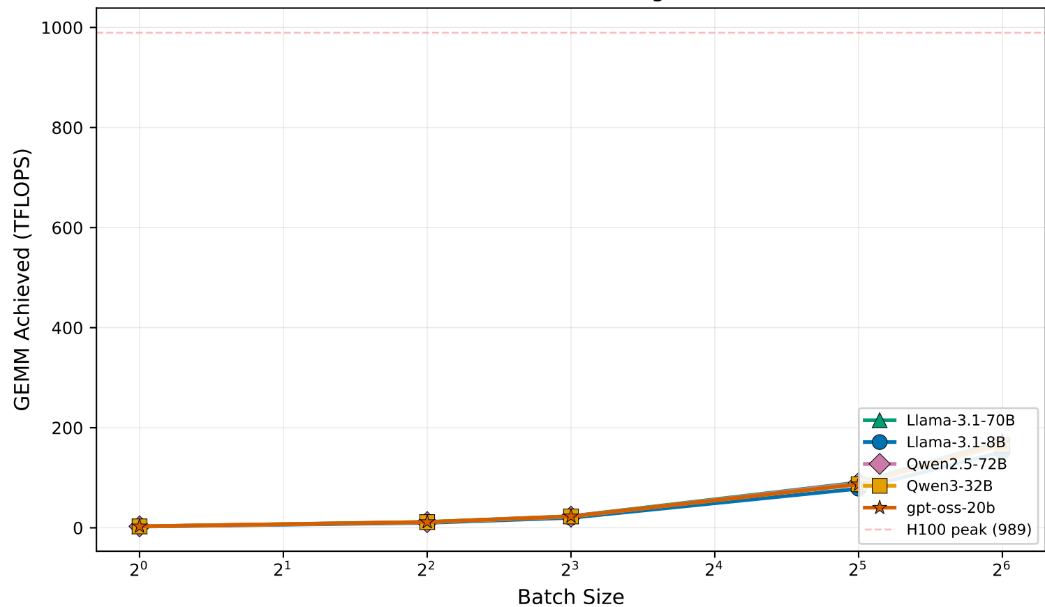
GEMM Performance Scaling — decode
