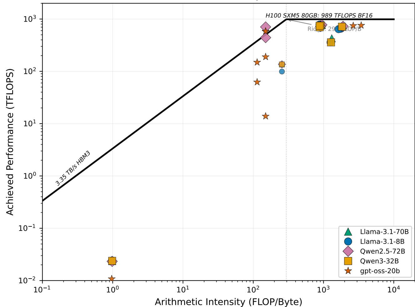
Cross-Model Roofline — prefill (BS=1)
