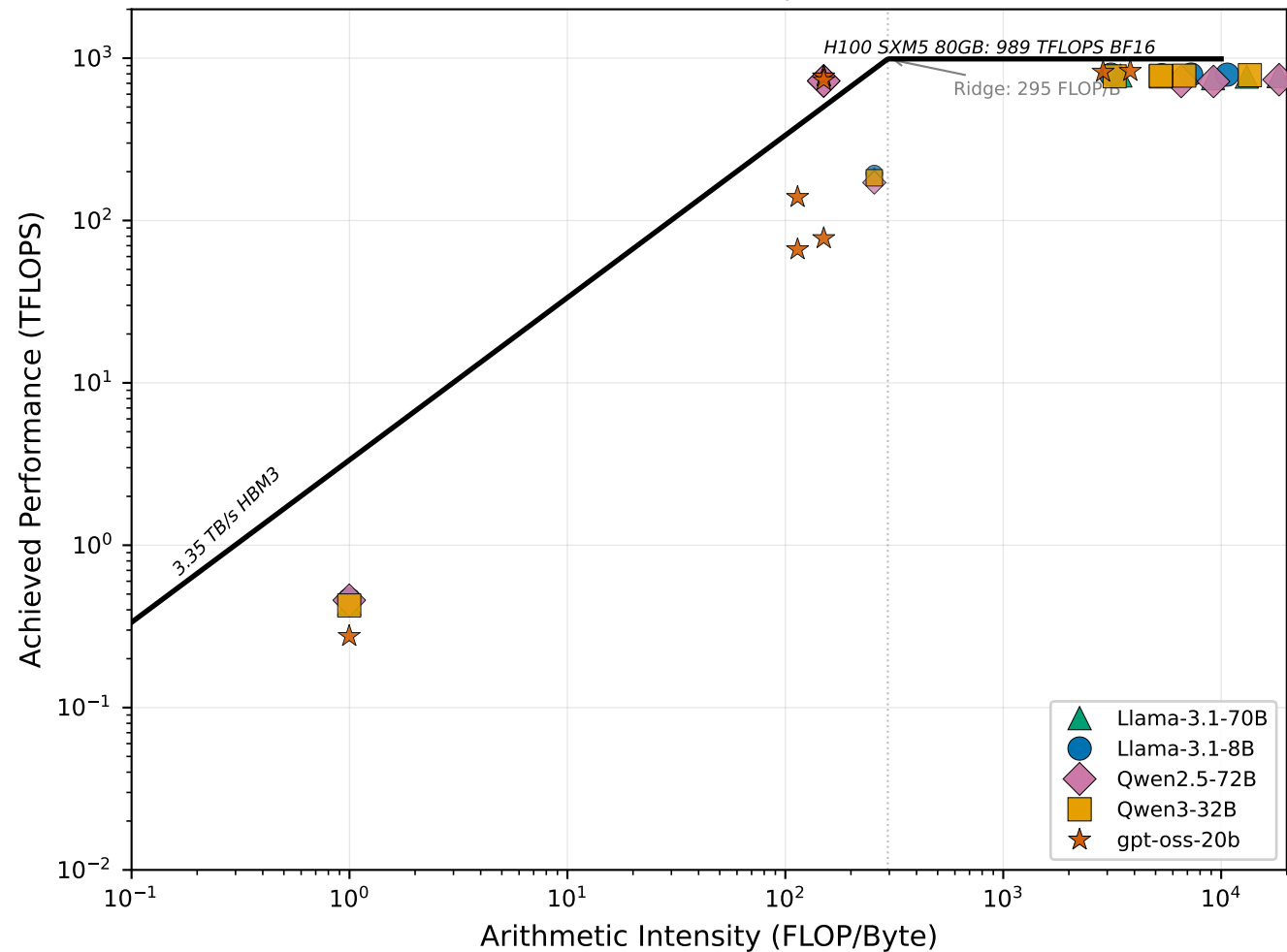
Cross-Model Roofline — prefill (BS=32)
