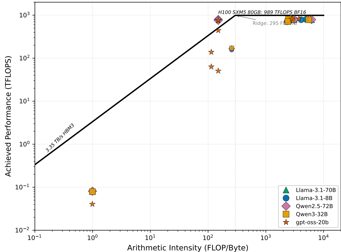
Cross-Model Roofline — prefill (BS=4)
