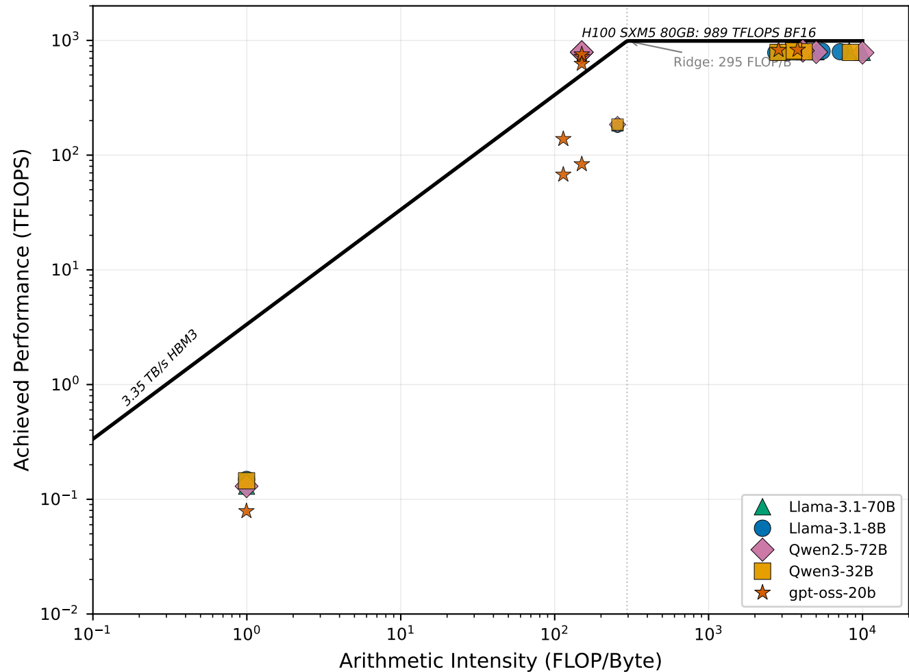
Cross-Model Roofline — prefill (BS=8)
