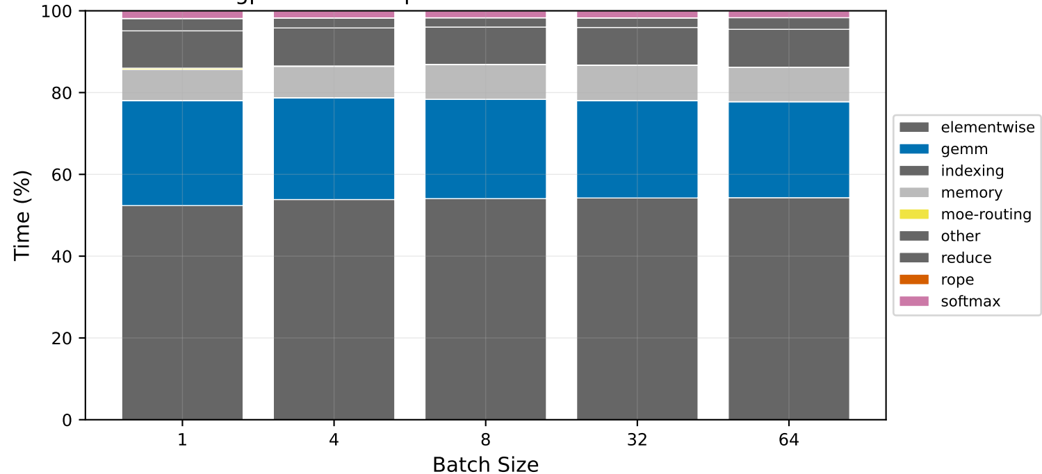
gpt-oss-20b — prefill Kernel Time Breakdown
