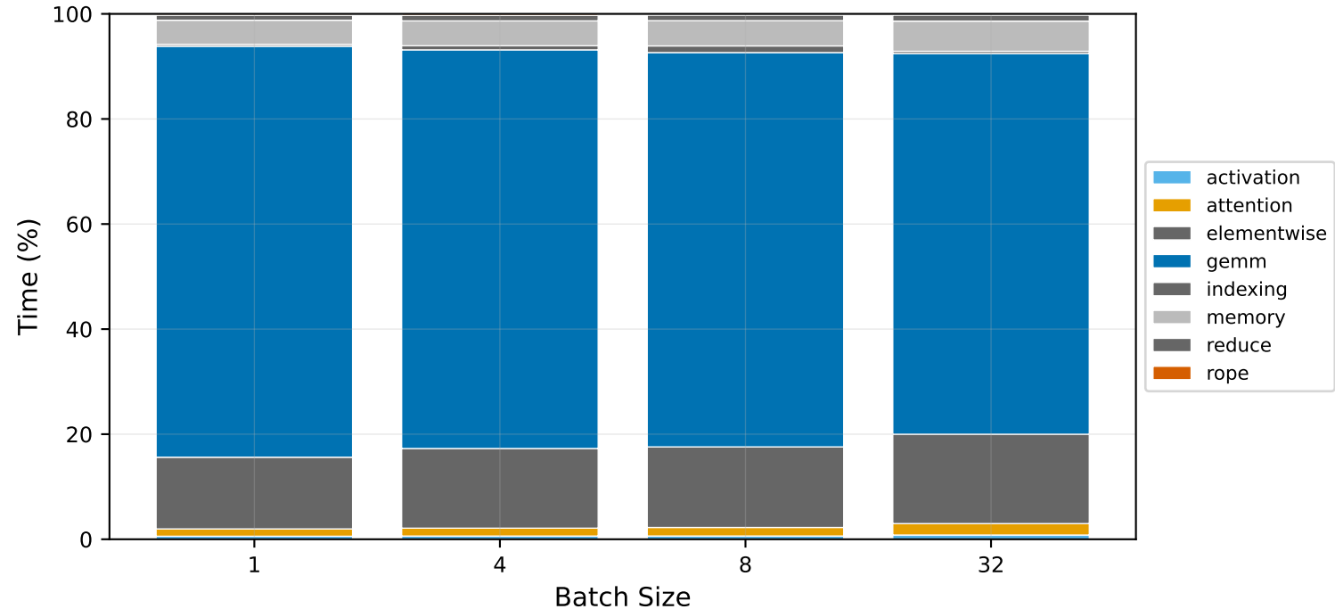
Llama-3.1-70B-Instruct — decode Kernel Time Breakdown
