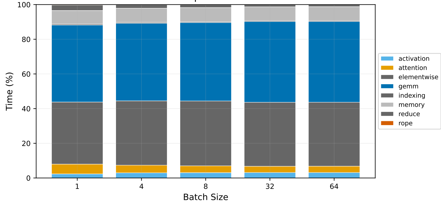
Llama-3.1-8B-Instruct — prefill Kernel Time Breakdown
