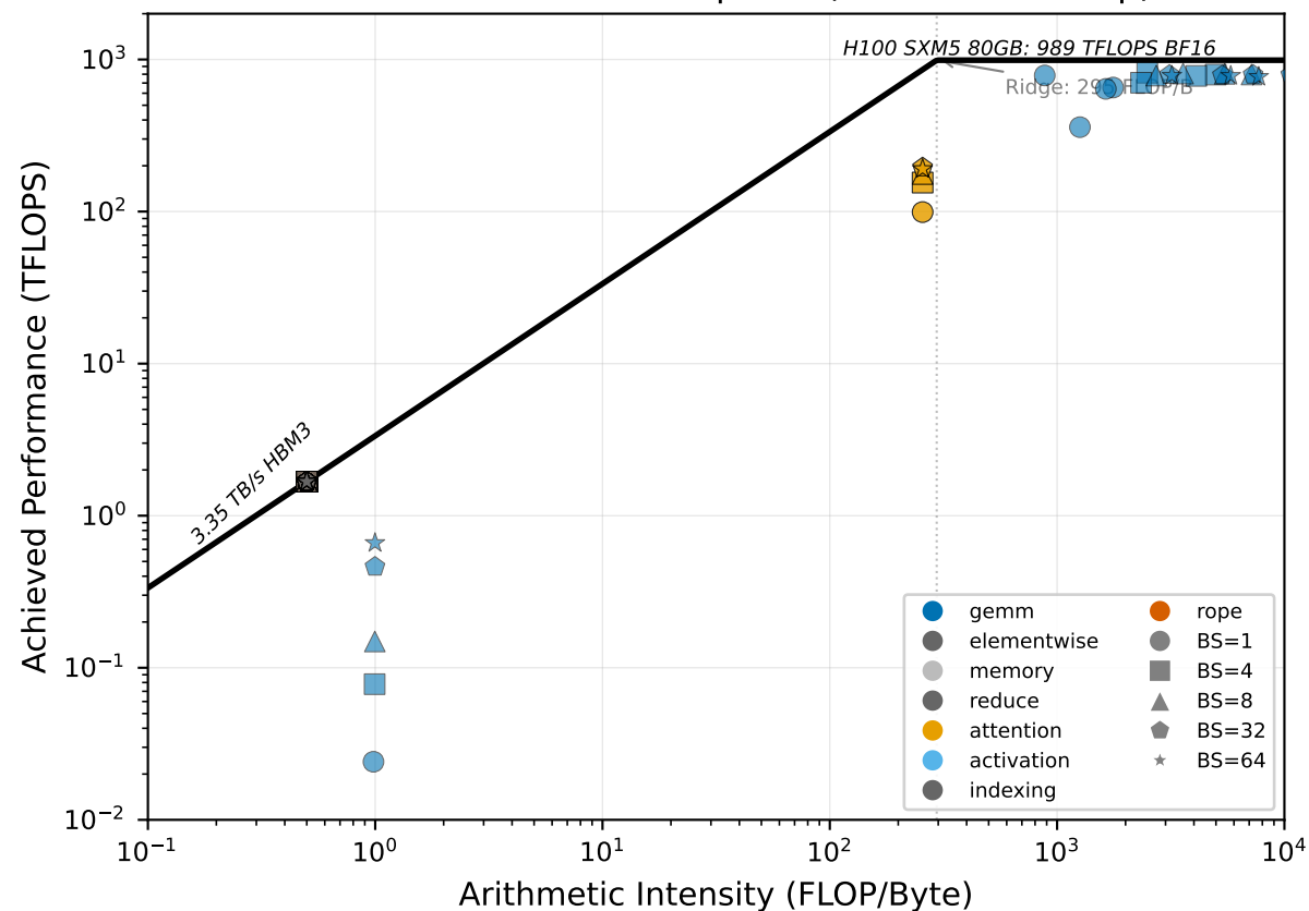
Llama-3.1-8B-Instruct — prefill (batch size sweep)
