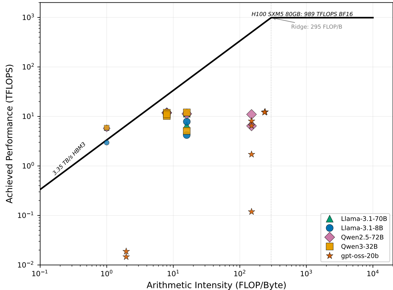
Cross-Model Roofline — decode (BS=4)
