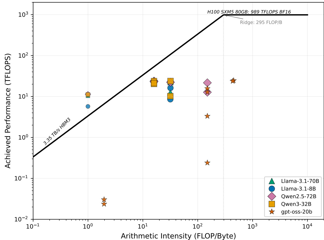
Cross-Model Roofline — decode (BS=8)
