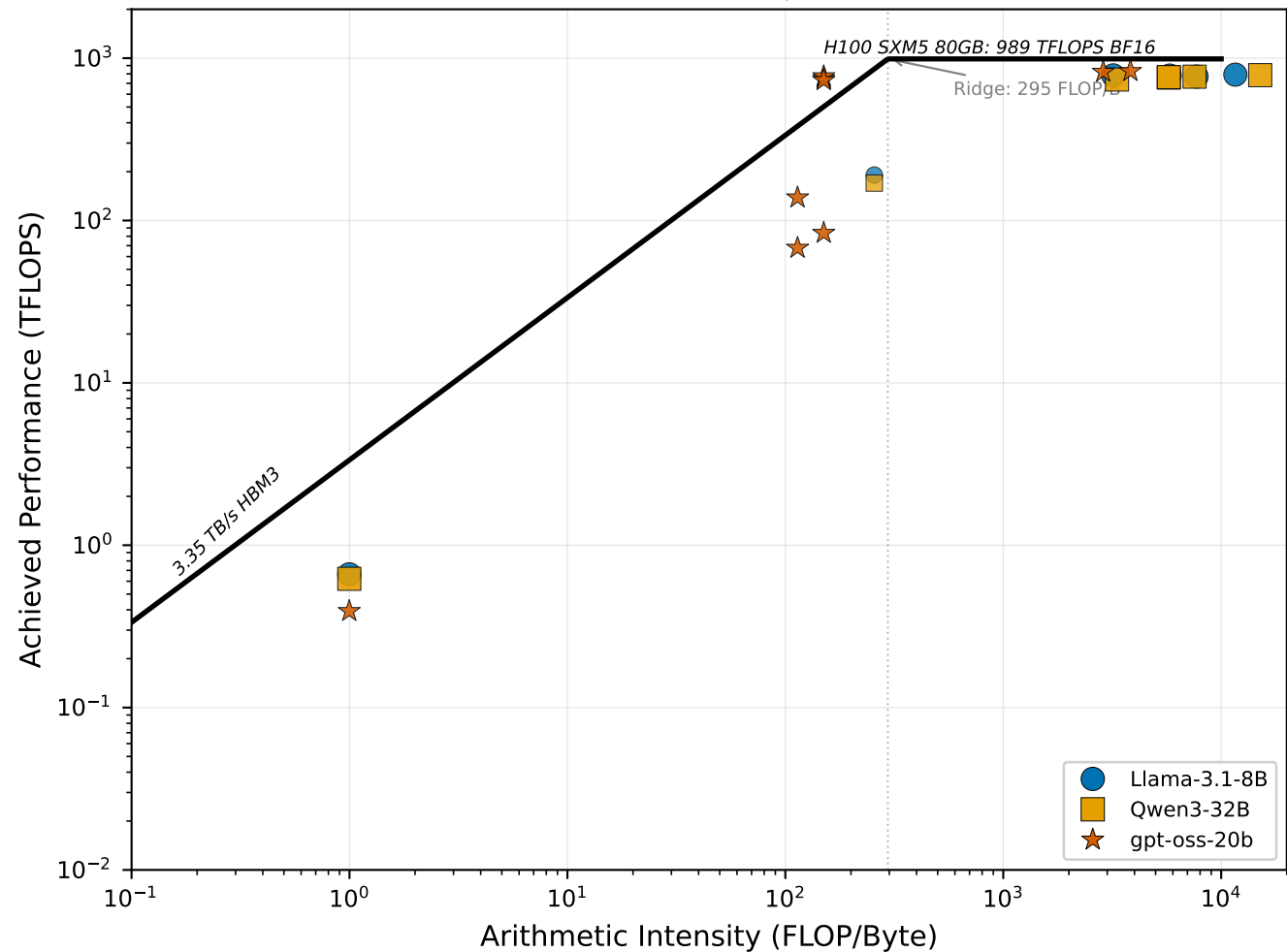
Cross-Model Roofline — prefill (BS=64)
