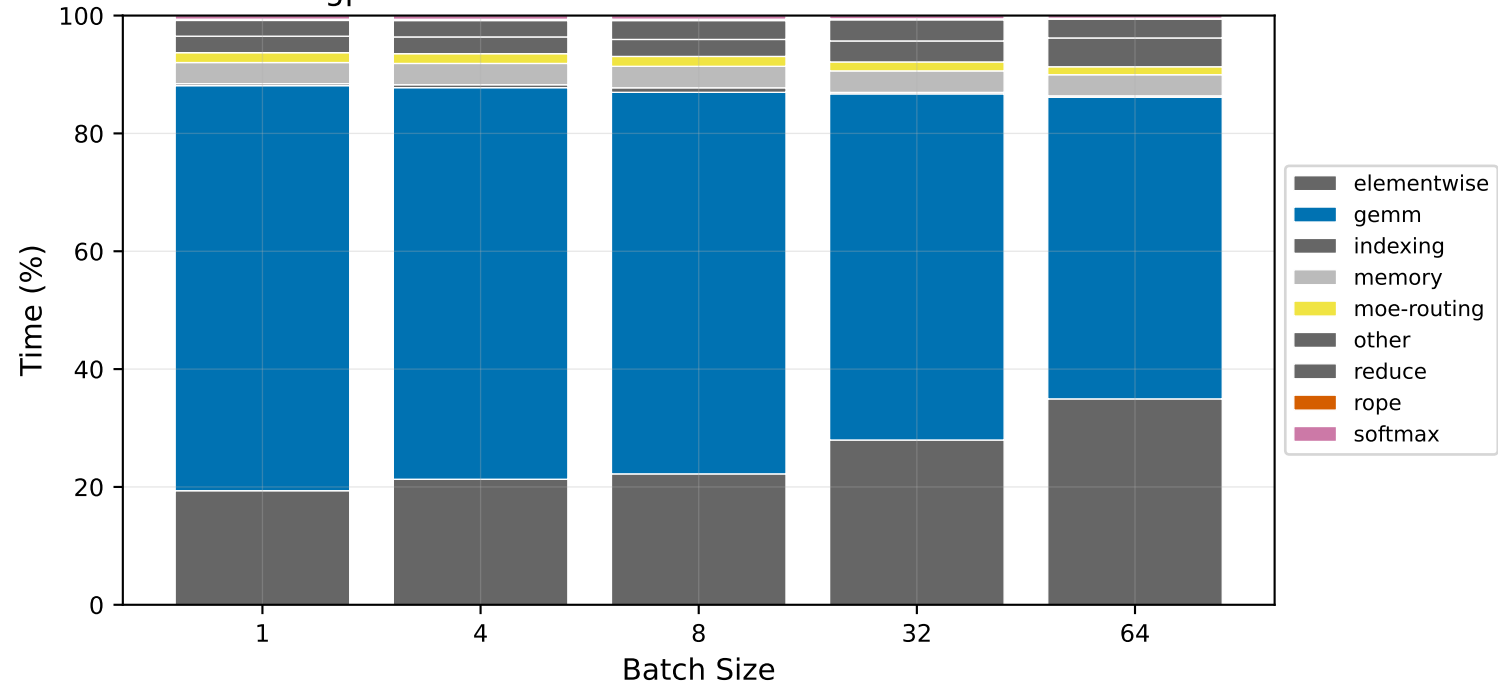
gpt-oss-20b — decode Kernel Time Breakdown
