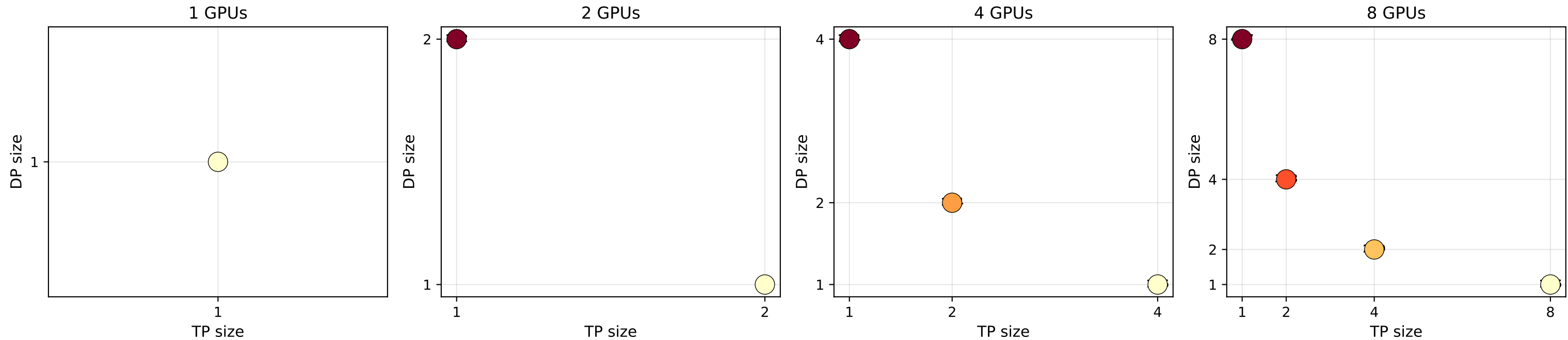
Llama-3.1-8B — Throughput (samples/s) by TP×DP
