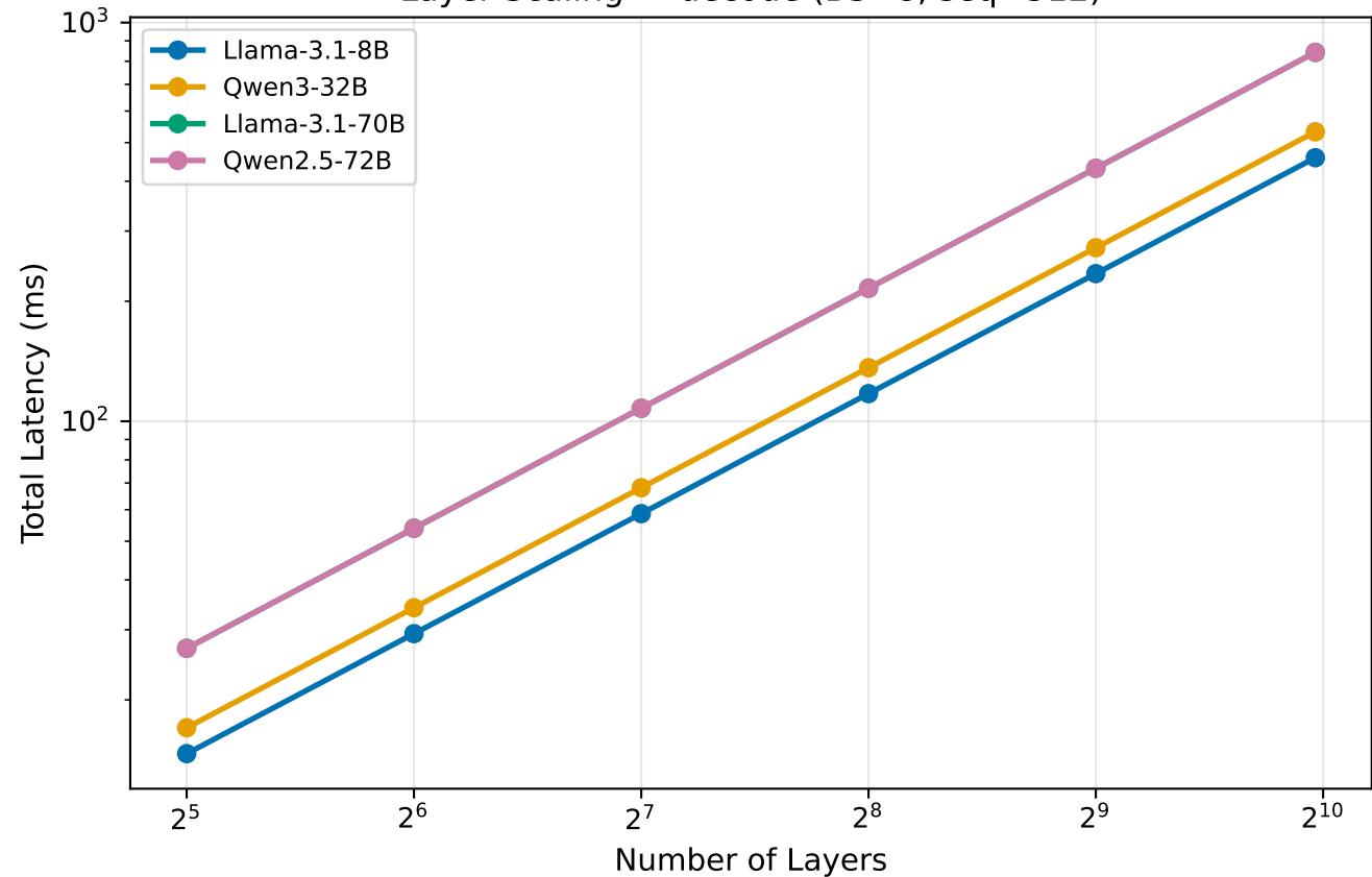
Layer Scaling — decode (BS=8, seq=512)
