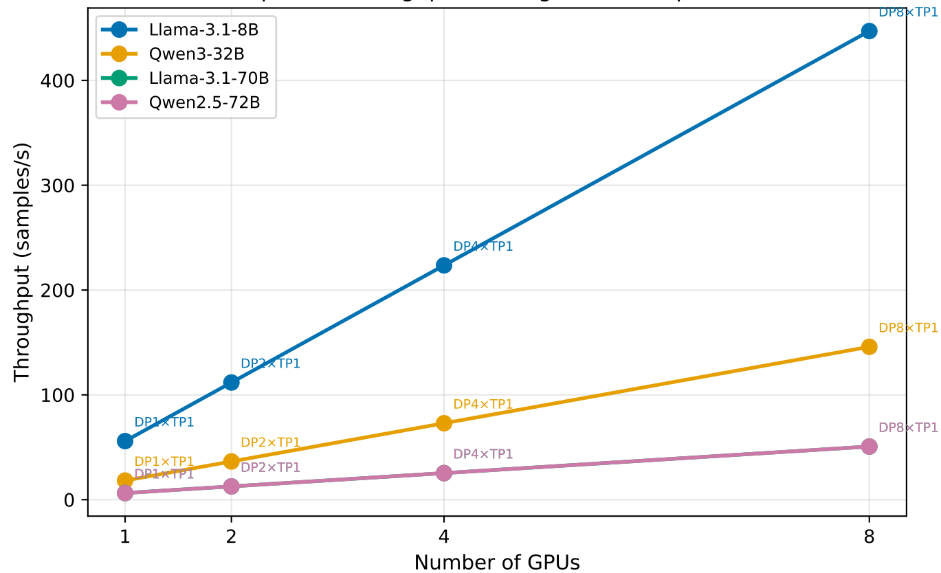
Optimal Throughput Scaling (BS=8, seq=512)
