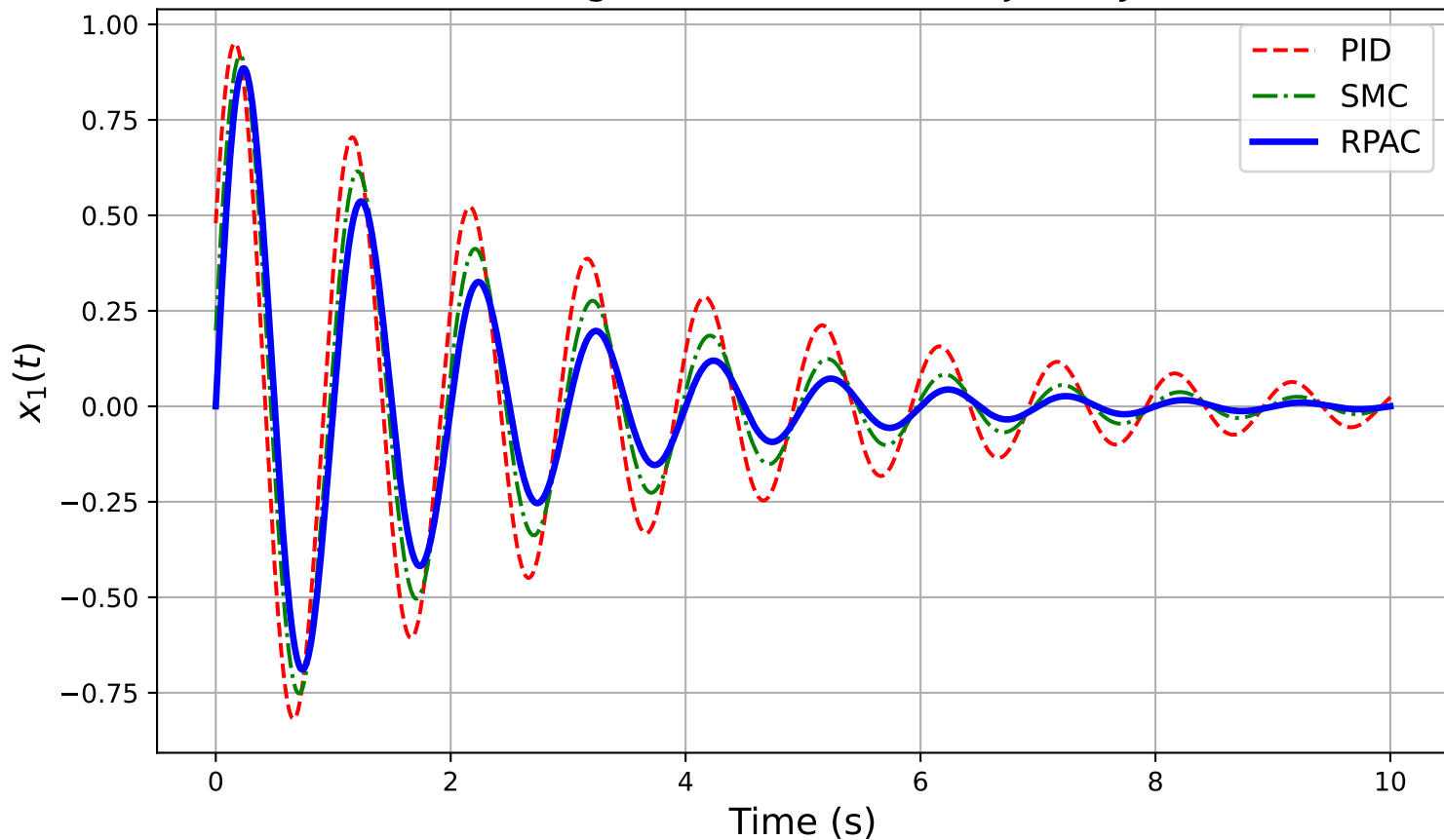
Duffing Oscillator: State Trajectory
