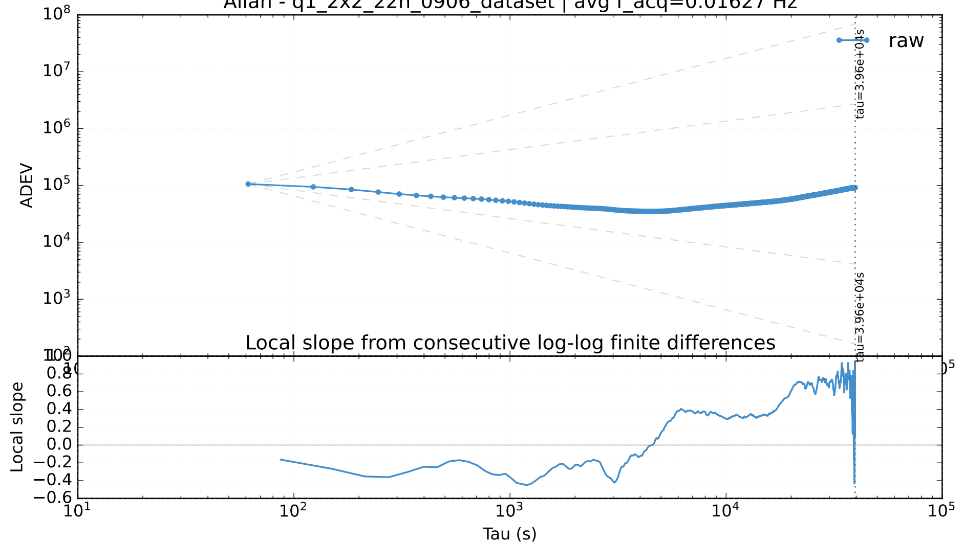
Allan - q1_2x2_22h_0906_dataset | avg f_{\text{acq}}=0.01627 Hz
