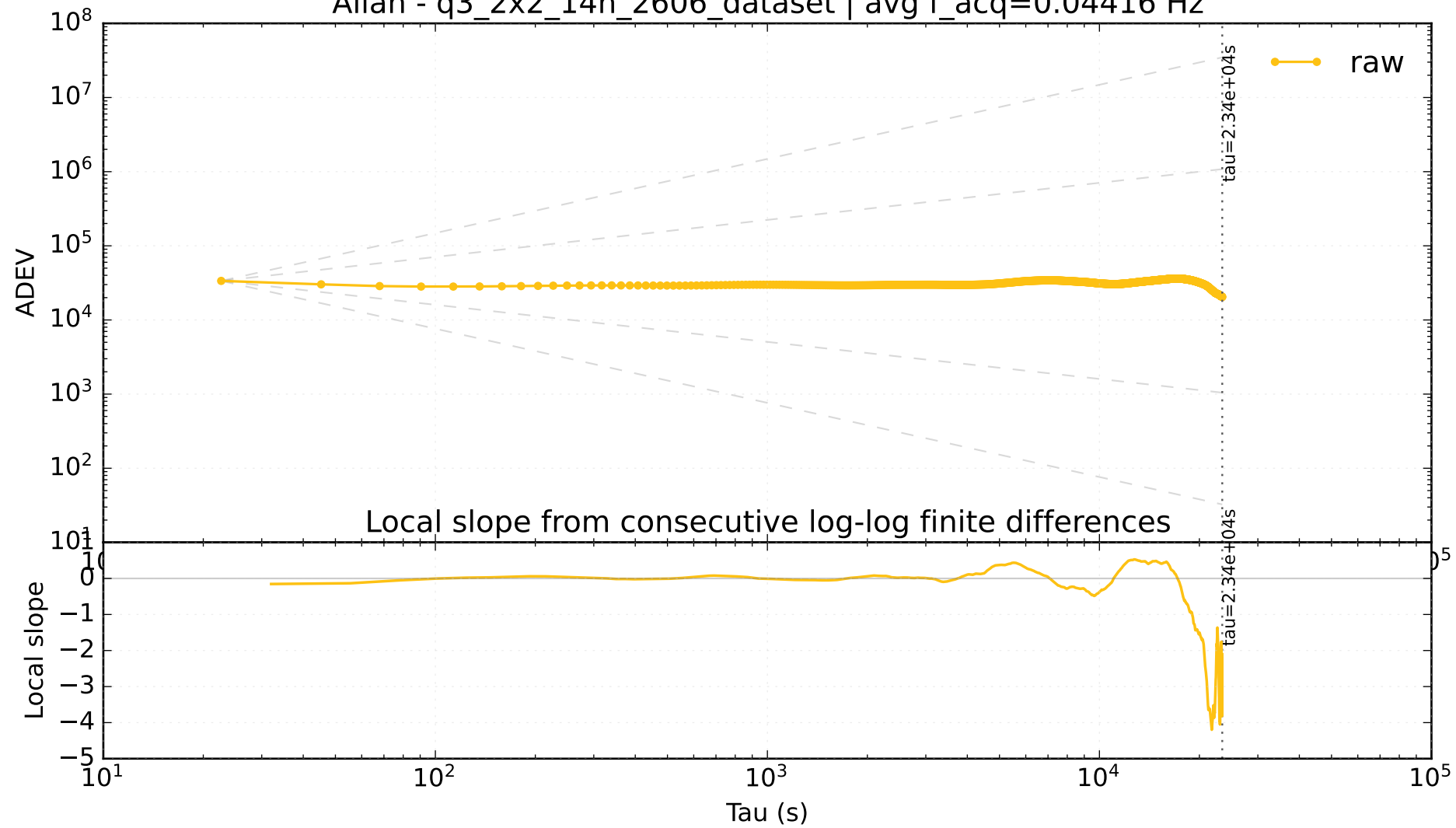
Allan - q3 2x2 14h 2606 dataset | avg f acq=0.04416 Hz
