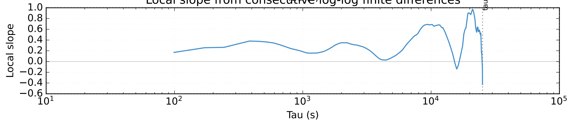
Local slope from consecutive log-log finite differences
