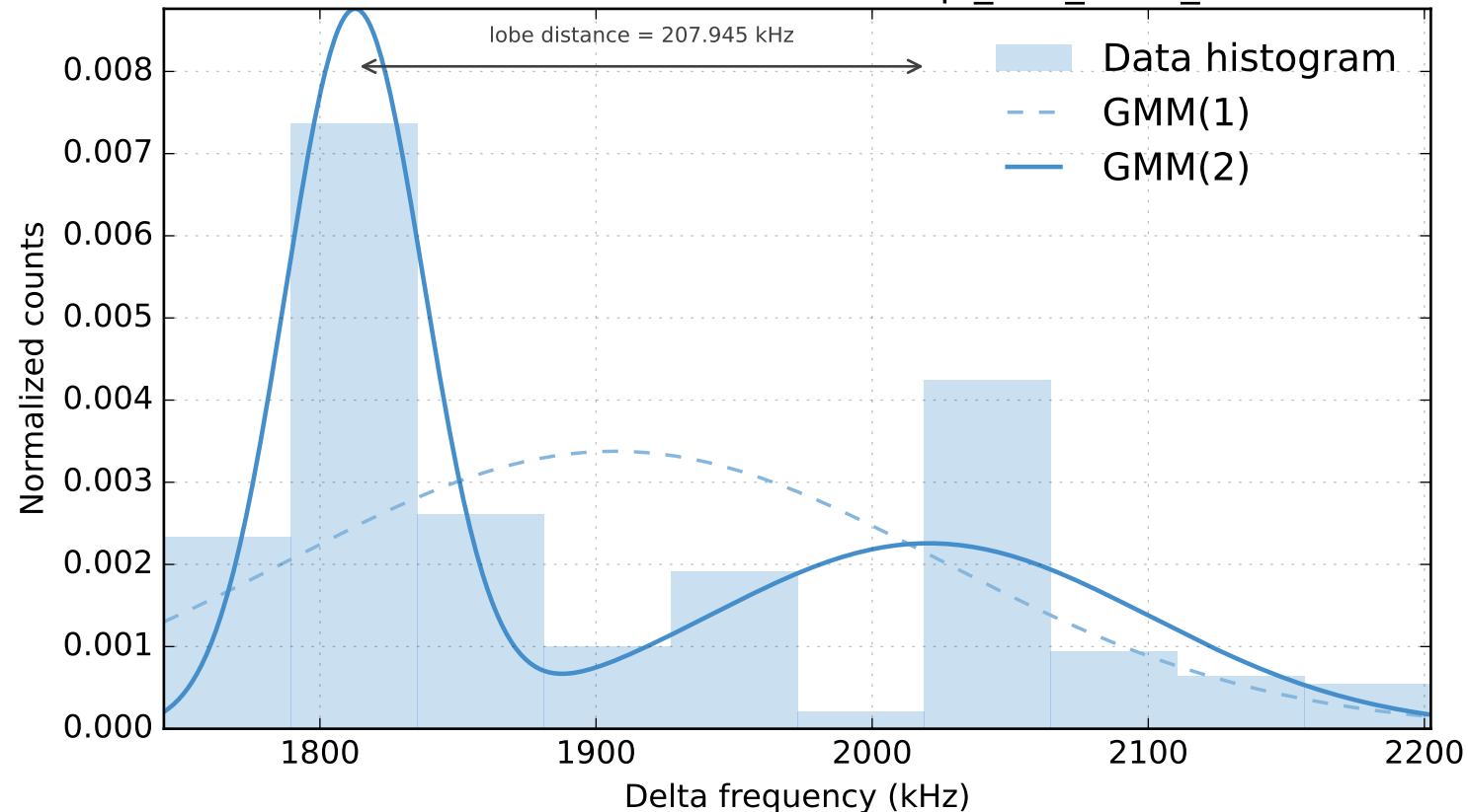
TLF distribution and Gaussian fits - q1_14h_1204_dataset
