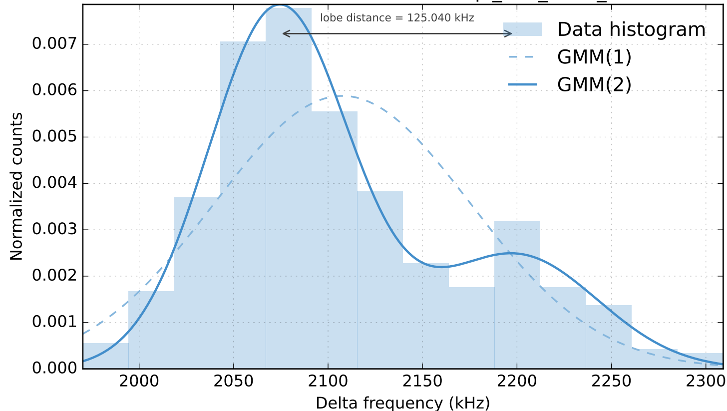
TLF distribution and Gaussian fits - q1_14h_2104_dataset
