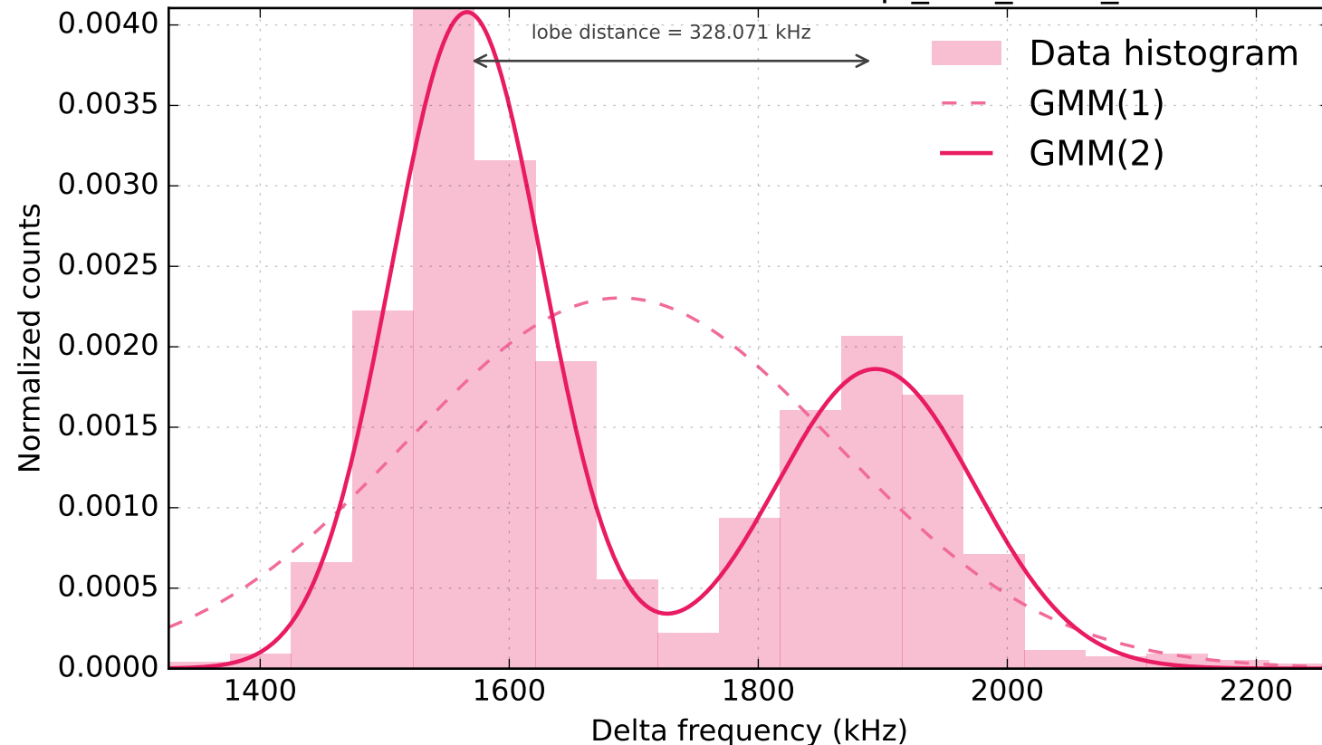
TLF distribution and Gaussian fits - q2_12h_2806_dataset
