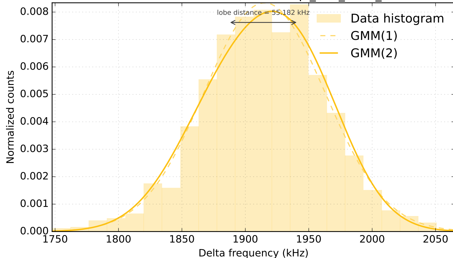
TLF distribution and Gaussian fits - q3_15h_1107_dataset
