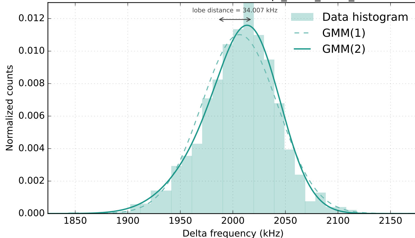
TLF distribution and Gaussian fits - q4_100h_0707_dataset
