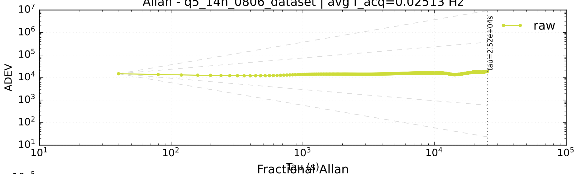
Allan - q5_14h_0806_dataset | avg f_acq=0.02513 Hz
