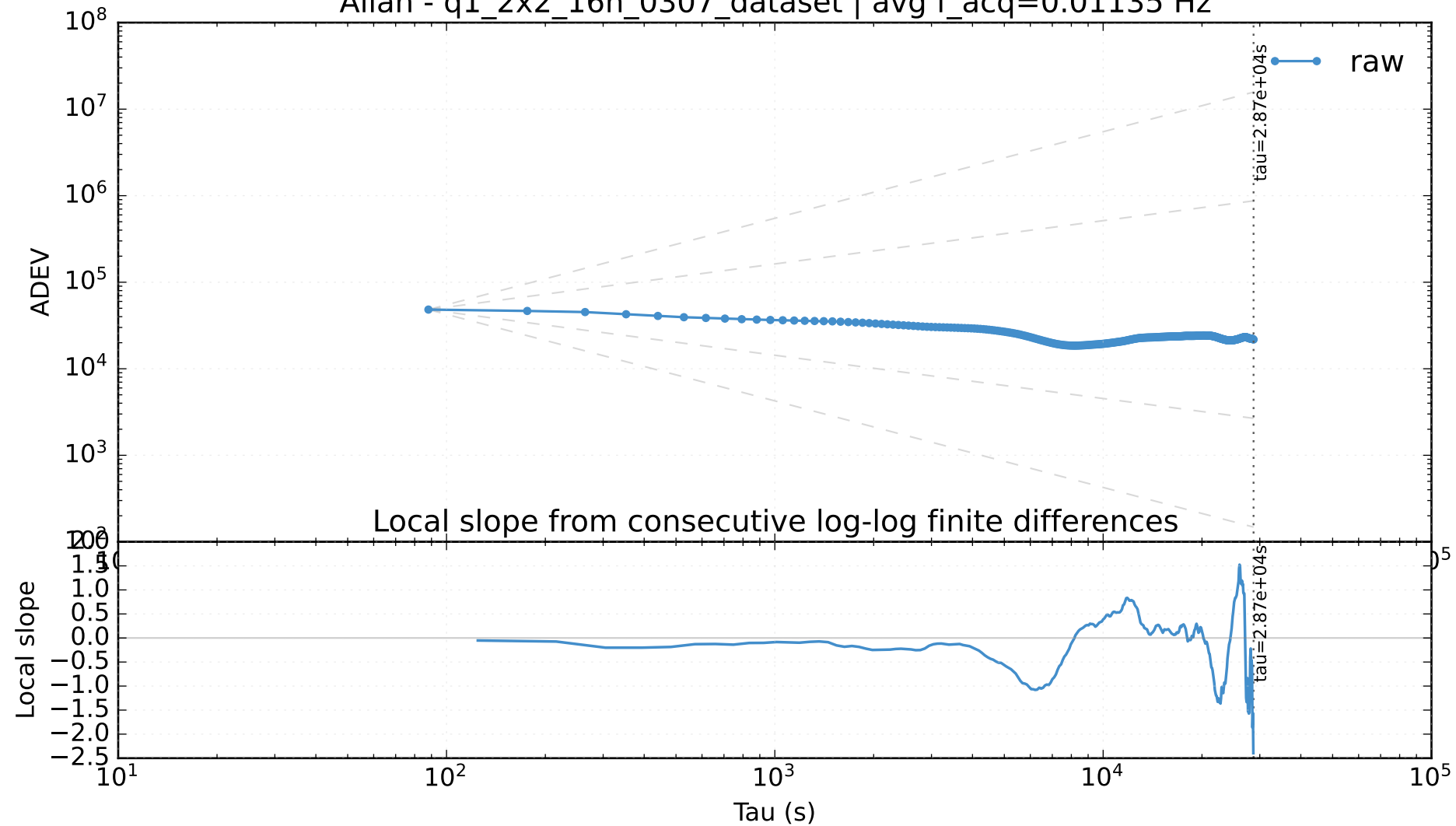
Allan - q1_2x2_16h_0307_dataset | avg f_acq=0.01135 Hz
