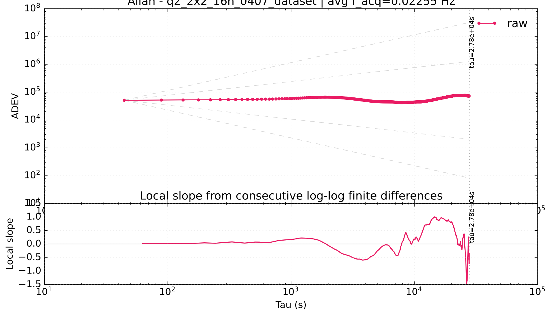
Allan - q2_2x2_16h_0407_dataset | avg f_acq=0.02255 Hz
