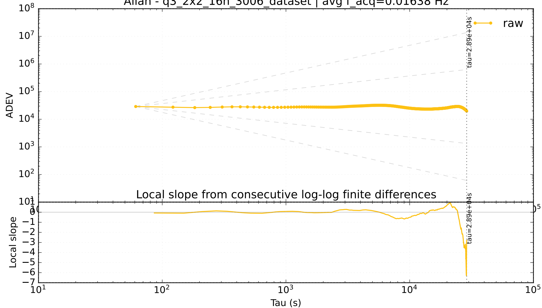
Allan - q3_2x2_16h_3006_dataset | avg f_acq=0.01638 Hz
