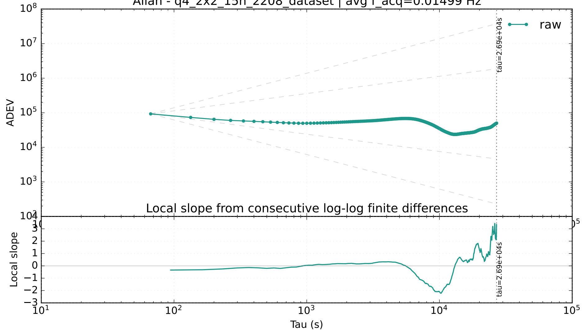
Allan - q4_2x2_15h_2208_dataset | avg f_{\text{acq}}=0.01499 Hz
