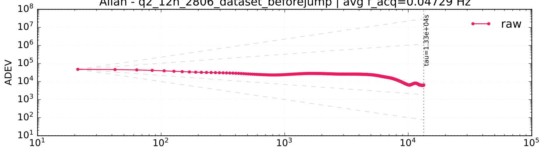
Fractional Allan
