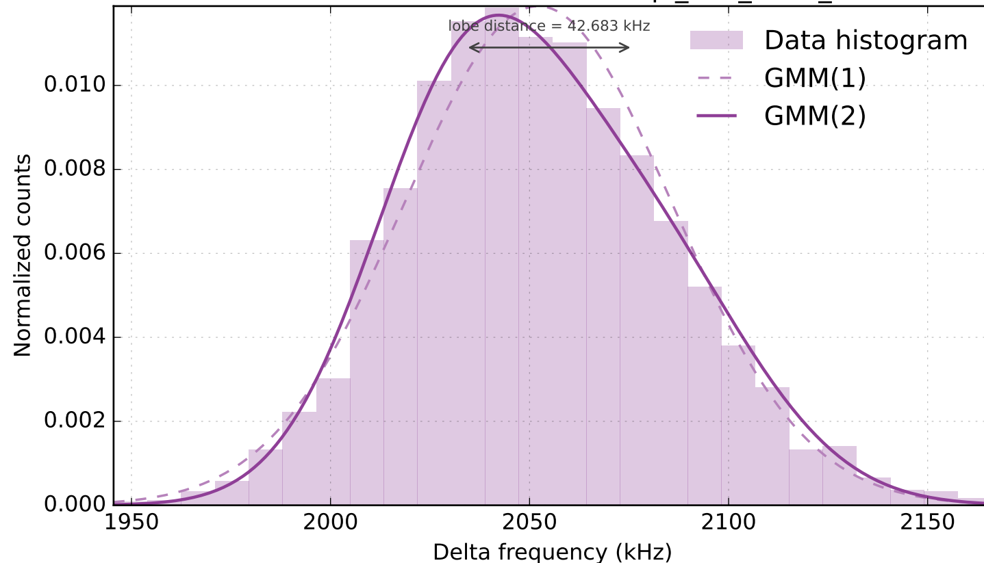
TLF distribution and Gaussian fits - q6_39h_0906_dataset
