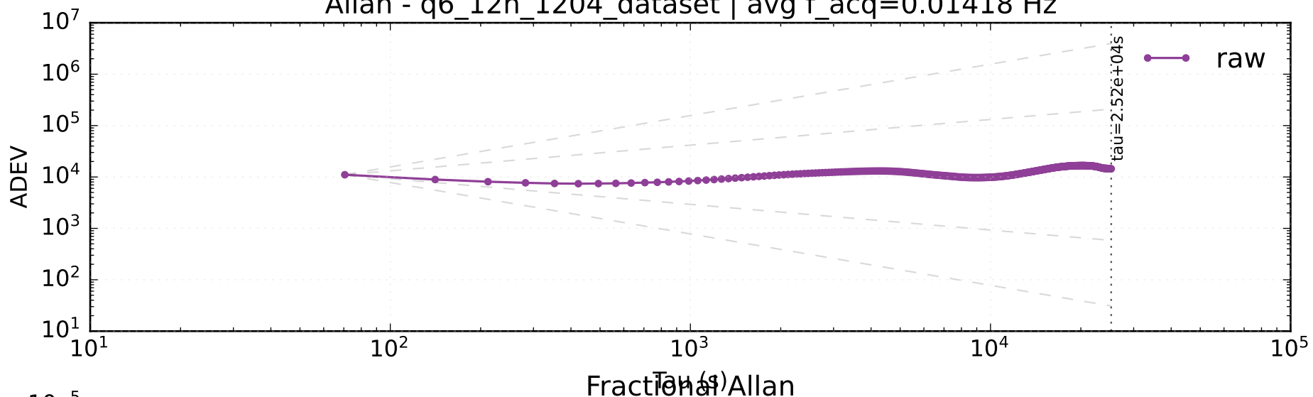
Allan - q6_12h_1204_dataset | avg f_acq=0.01418 Hz
