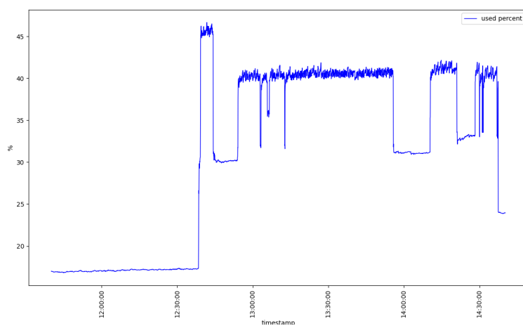
Figure 3: RAM percent
