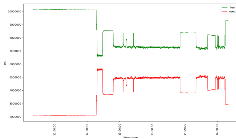
Figure 2: RAM absolute
