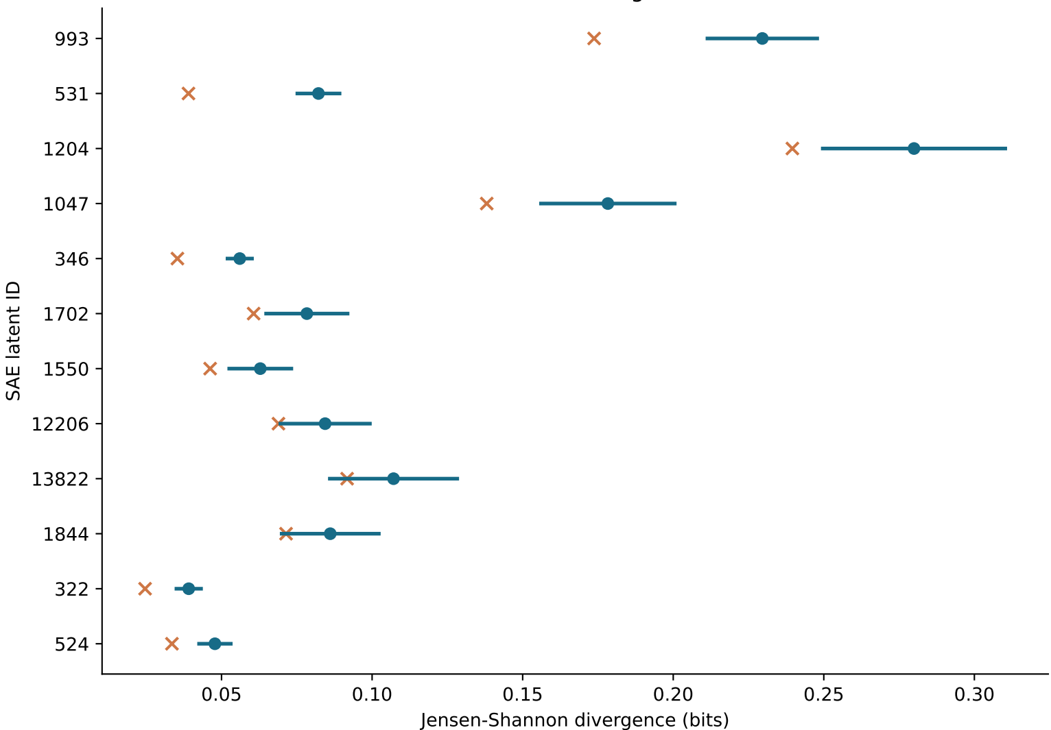
Observed effects and document-bootstrap intervals Blue: observed / 95% interval; orange: mean conditional null
