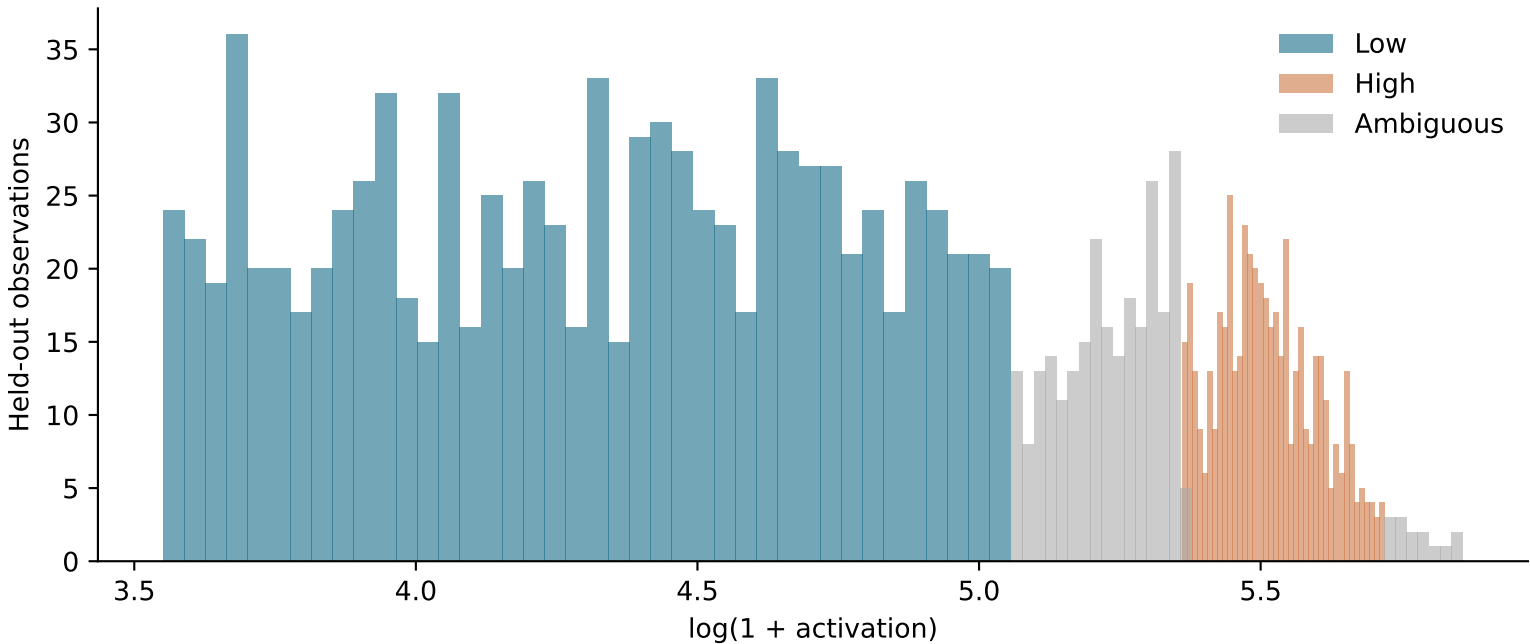
Latent 993: frozen discovery GMM assignments (delta BIC 720.5)
