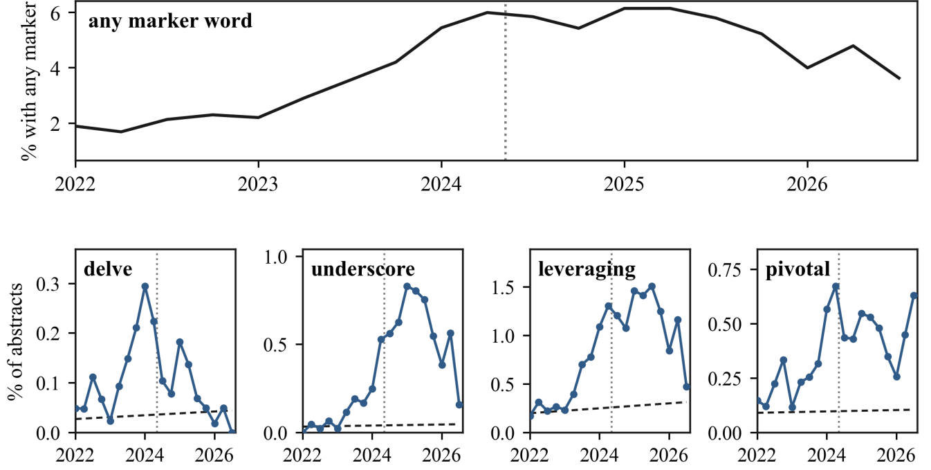
Figure A1. Top: the fraction of abstracts with any marker word, by quarter. Bottom: four individual words, each on its own scale. The dashed black segment in each panel extrapolates that word’s 2015–2021 linear trend. The vertical dotted line marks mid-2024, when delve received wide public attention as a sign of model-generated text. Its frequency declines from that point while the other markers continue to rise, and the aggregate rate does not fall.
