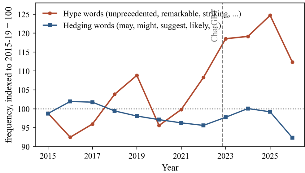
Figure A6. Promotional and hedging word frequency, indexed to the 2015–2019 mean. Promotional words rise together with the marker rate, while hedging words stay flat.
