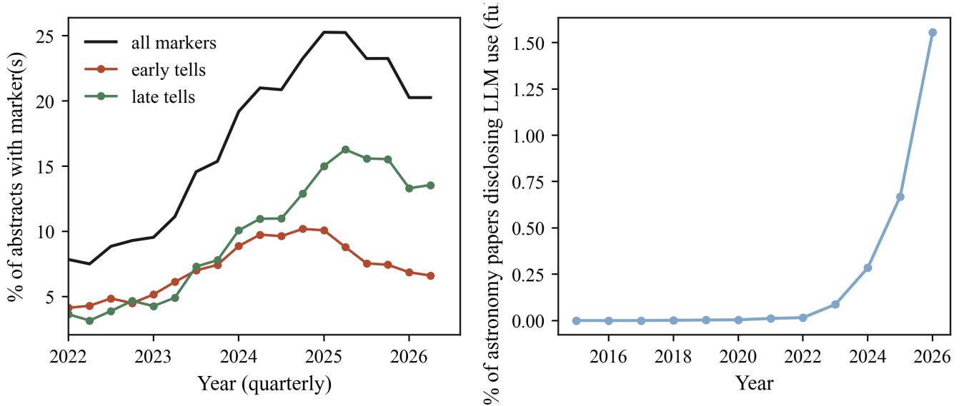
Figure 7. Left: the marker words weaken across the board in 2026, both the early markers that peaked first ( delve , intricate , pivotal ) and the later ones ( underscore , leveraging ). Right: over the same months, stated model use continues to rise.
