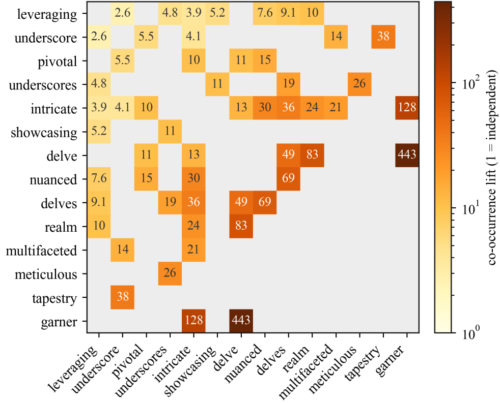
Figure 3. Co-occurrence lift for pairs of marker words in 2024–2026 abstracts. Colored cells are the 27 of 91 pairs whose joint count exceeds the independence expectation at p < 0.01 (Poisson test). Grey cells are consistent with independence. Lifts above \sim 40 rest on one to three joint abstracts and are order-of-magnitude values.
