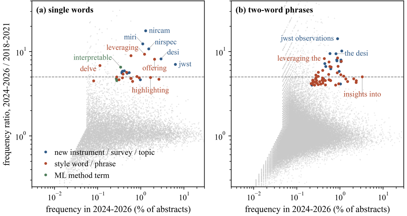
Figure 2. Frequency ratio between 2024–2026 and 2018–2021 against recent frequency for (a) every word and (b) every two-word phrase in the corpus (grey points). The tail above the dashed line at ratio 5 splits into new instruments, surveys, and topics (blue), style words and phrases (red), and technical machine-learning terms (green), and selected items are labeled. Axes are logarithmic.
