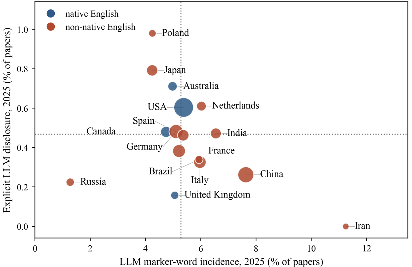
Figure 6. Marker rate against disclosure rate by author country in 2025. Blue points mark countries where English is a first language, and bubble size is the number of papers. Wilson 95% intervals on the marker rates are quoted in the text. The smallest sample shown is Iran with n = 418 . The affiliation search counts every country on a paper, so large collaborations enter more than once.
