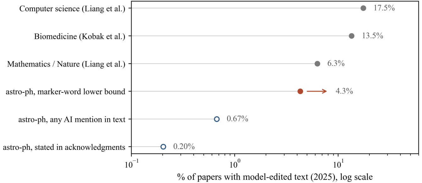
Figure 4. The model-touched fraction of 2025 papers across fields and detection routes, on a logarithmic axis. Grey points are published estimates for other fields (Liang et al. 2025; Kobak et al. 2025). The red point is our marker-word estimate for astro-ph, and the arrow marks it as a lower bound. Open circles are the fractions of astronomy papers that mention or state model use. The gap between the red point and the open circles separates use from disclosure.
