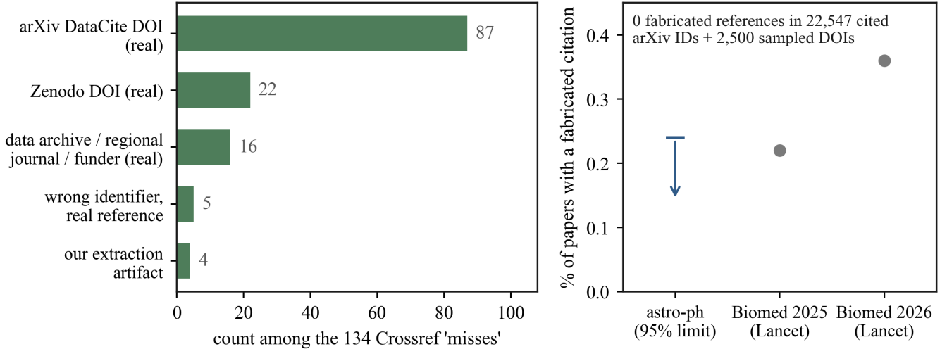
Figure 5. Left: classification, after manual inspection, of the 134 DOIs that a Crossref check could not resolve. None is a fabricated reference. Most are real records in registries Crossref does not index, five are wrong identifiers attached to real references, and four are artifacts of our extraction. Right: the fabricated-citation rate. The astronomy value is the 95% upper limit from zero detections (arrow), against the biomedical audit of Topaz et al. (2026).
