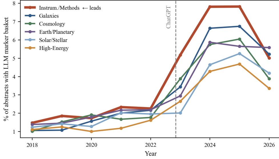
Figure 10. Marker rate by primary astro-ph subfield. Instrumentation and Methods leads; high-energy astrophysics trails.
