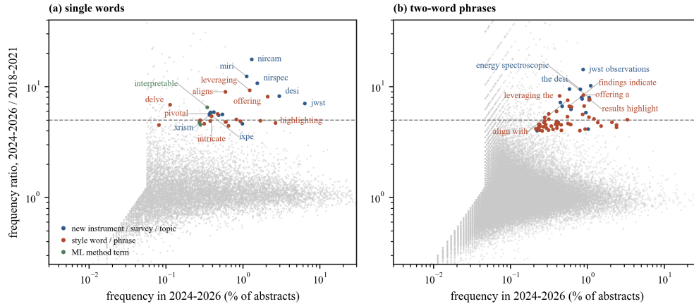
Figure 3. Frequency ratio between 2024–2026 and 2018–2021 against recent frequency for (a) every word and (b) every two-word phrase in the corpus (grey points). The tail above the dashed line at ratio 5 separates into new instruments, surveys, and topics (blue), style words and phrases (red), and technical machine-learning terms (green); selected items are labeled. Axes are logarithmic.
