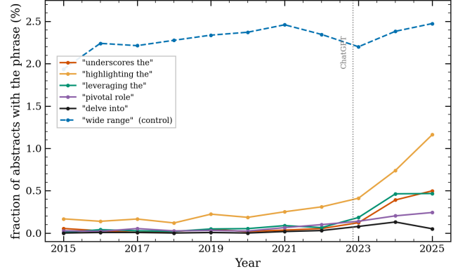
Figure 4. Fraction of abstracts containing selected two-word phrases, by year. Model-favored phrases rise after 2022; a control phrase ( wide range ) stays flat.
