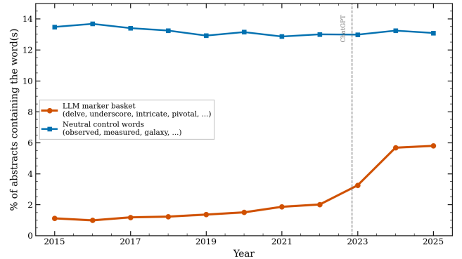
Figure 1. Fraction of astro-ph abstracts containing a marker word (red) and a matched set of neutral control words (blue), by year. The marker basket rises after ChatGPT while the control stays flat. Both are per-abstract fractions, so we stop at the last full year, 2025.
