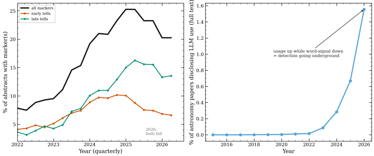
Figure 14. Left: the marker words weaken across the board in 2026, both the early tells that peaked first ( delve , intricate , pivotal ) and the later ones ( underscore , leveraging ). Right: over the same months, stated model use keeps rising. Use is not falling; the word signal is.
