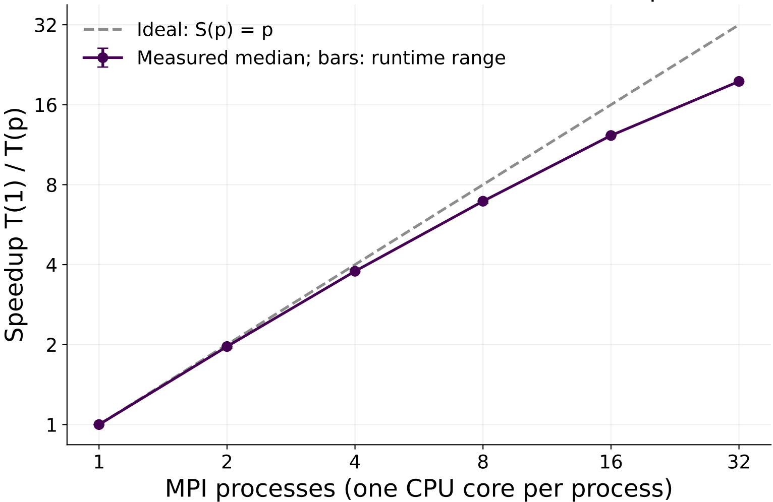
bwUniCluster: 64 × 64, 150,000 timesteps
