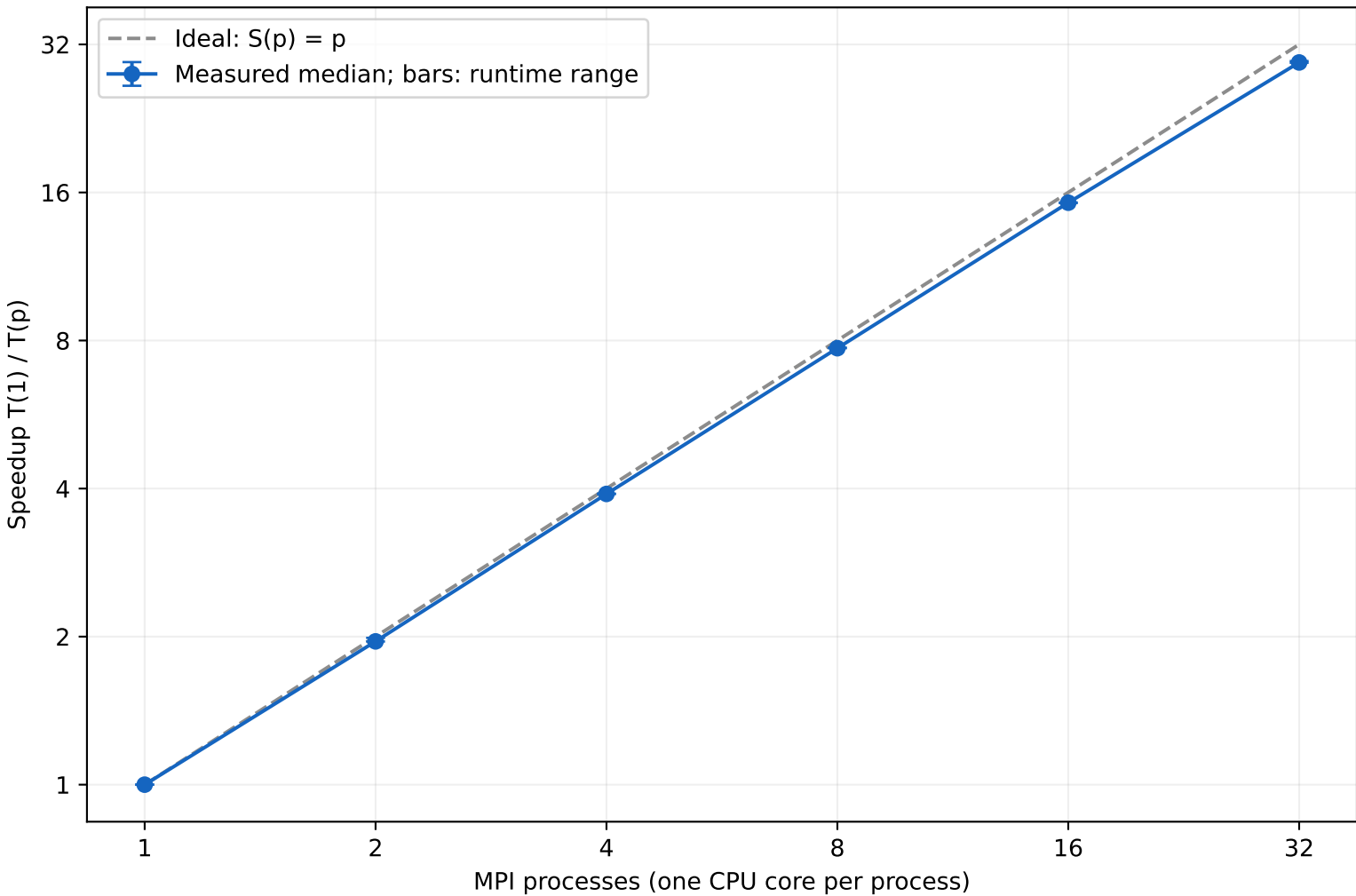
bwUniCluster: 256 \times 256 , 20,000 timesteps
