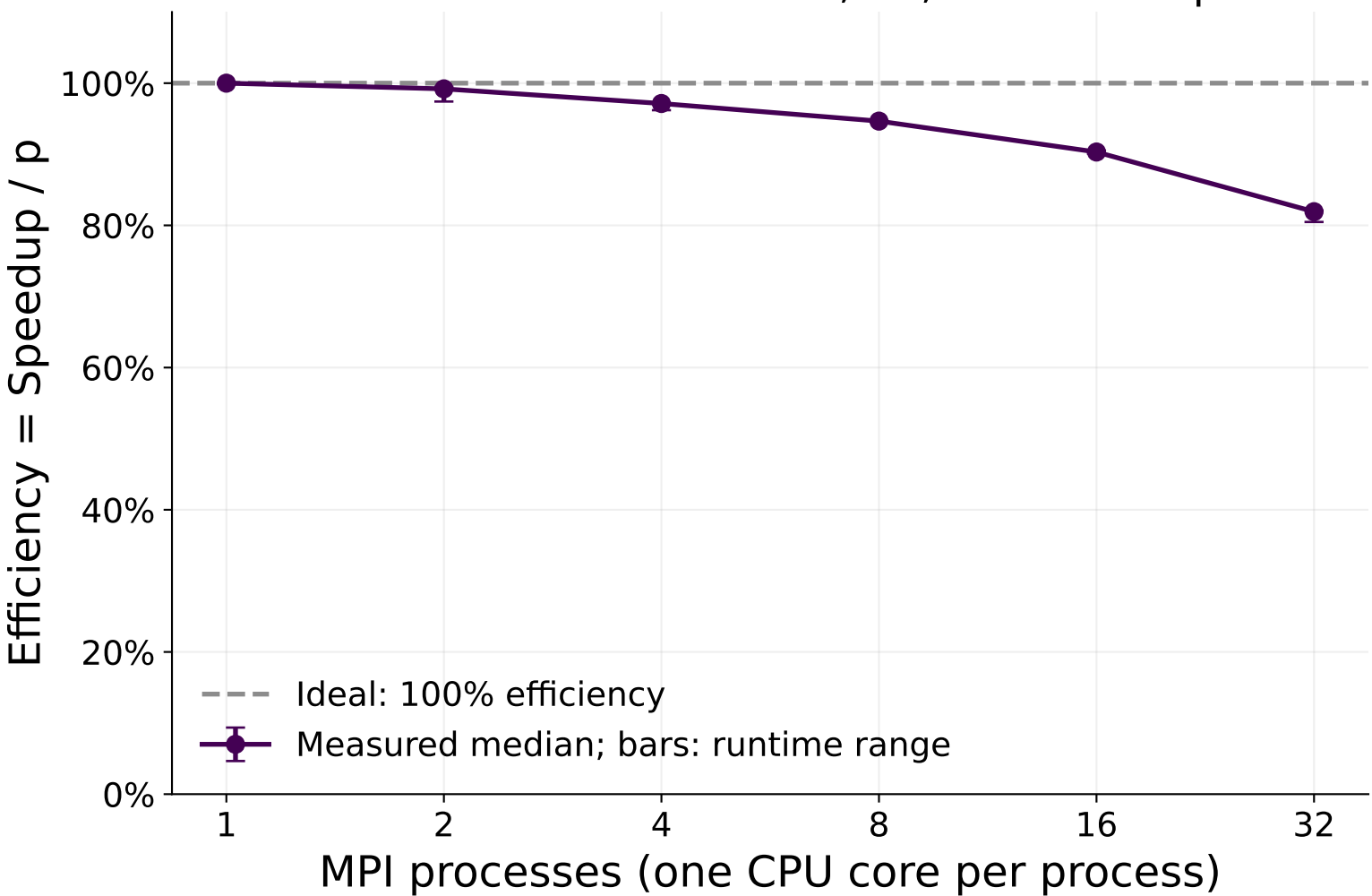
bwUniCluster: 128 × 128, 40,000 timesteps
