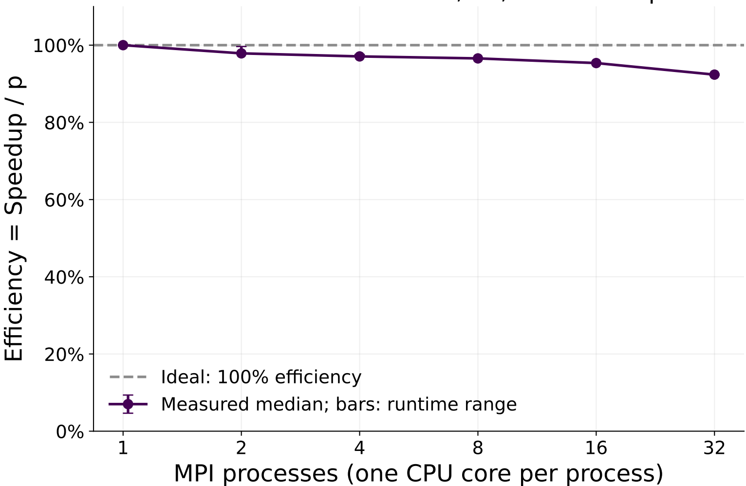
bwUniCluster: 256 × 256, 20,000 timesteps
