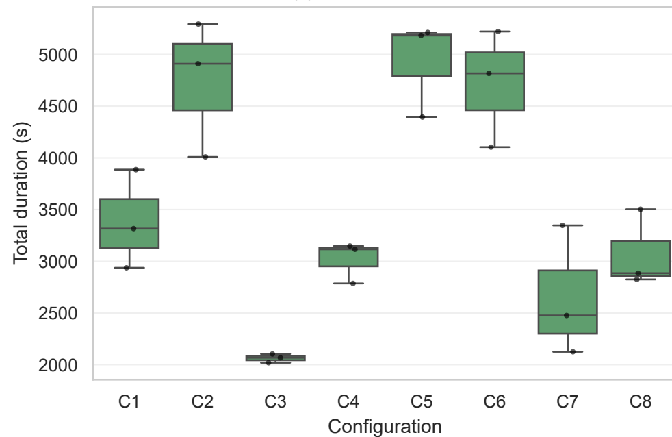
(c) Execution duration
